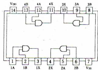
4081B
