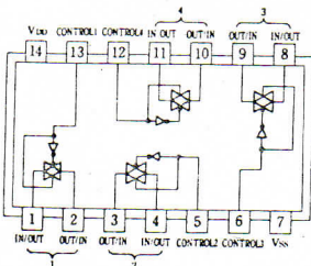
4066B
