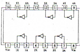
4049UB
